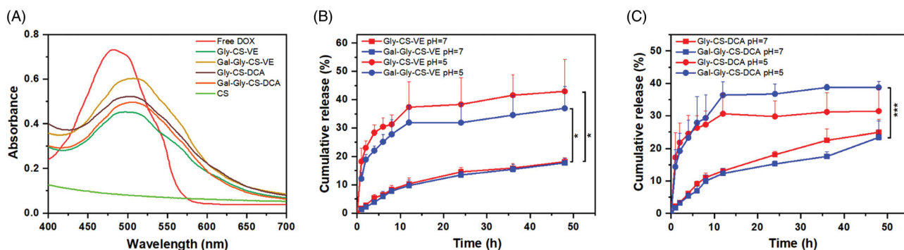
Figure 3. (A) UV-Vis absorption spectra of DOX solution, CS and DOX loaded chitosan nanoparticles. (B) In vitro release of DOX from Gly-CS-VE and Gal-Gly-CS-VE nanoparticles at pH 5 and 7. (C) In vitro release of DOX from Gly-CS-DCA and Gal-Gly-CS-DCA nanoparticles at pH 5 and 7, * p < 0.05 , *** p < 0.001 .
