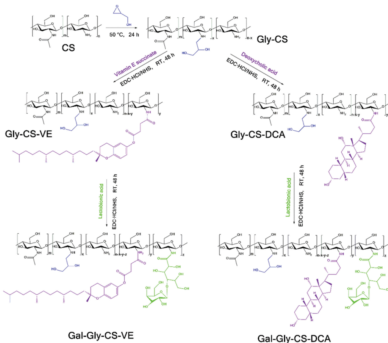
Figure 1. Synthetic scheme of chitosan derivatives (Gly-CS, Gly-CS-VE, Gal-Gly-CS-VE, Gly-CS-DCA, and Gal-Gly-CS-DCA).
