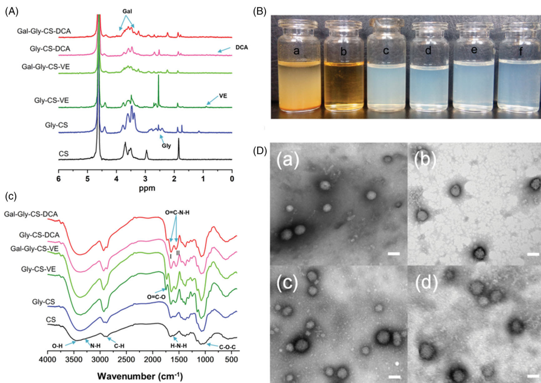
Figure 2. Characterizations of chitosan derivatives and nanoparticles. (A) ^1\text{H} NMR spectra of chitosan derivatives. (B) Appearance of aqueous solutions: (a) CS, (b) Gly-CS, (c) Gly-CS-VE, (d) Gal-Gly-CS-VE, (e) Gly-CS-DCA, (f) Gal-Gly-CS-DCA. (C) FT-IR spectra of chitosan derivatives. (D) TEM images of chitosan nanoparticles: (a) Gly-CS-VE, (b) Gal-Gly-CS-VE, (c) Gly-CS-DCA, (d) Gal-Gly-CS-DCA, scale bar = 100 nm.
